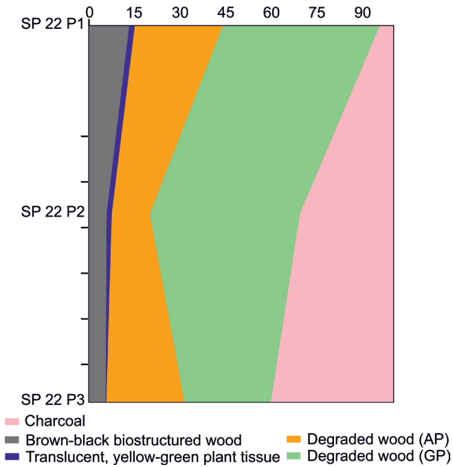
Figure 4. Phytoclasts ratio.
