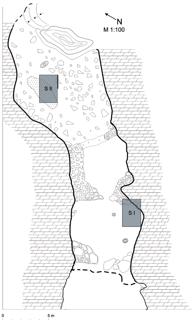
Figure 2. Plan of the Spila nad Procjepom cave with locations of the test pits Sonda I (S I) and Sonda II (S II). Sampled profile of S II is marked with a bold line.
